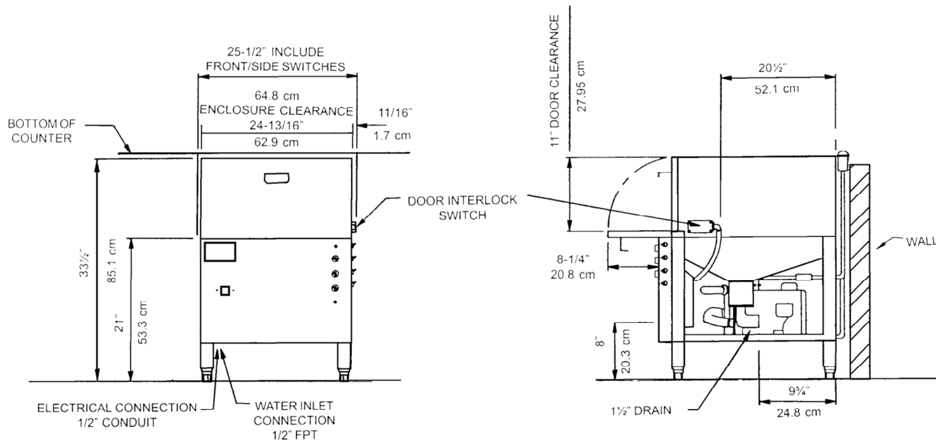
FRONT VIEW
